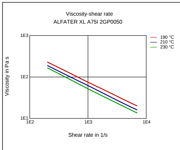
Viscosity-shear rate
